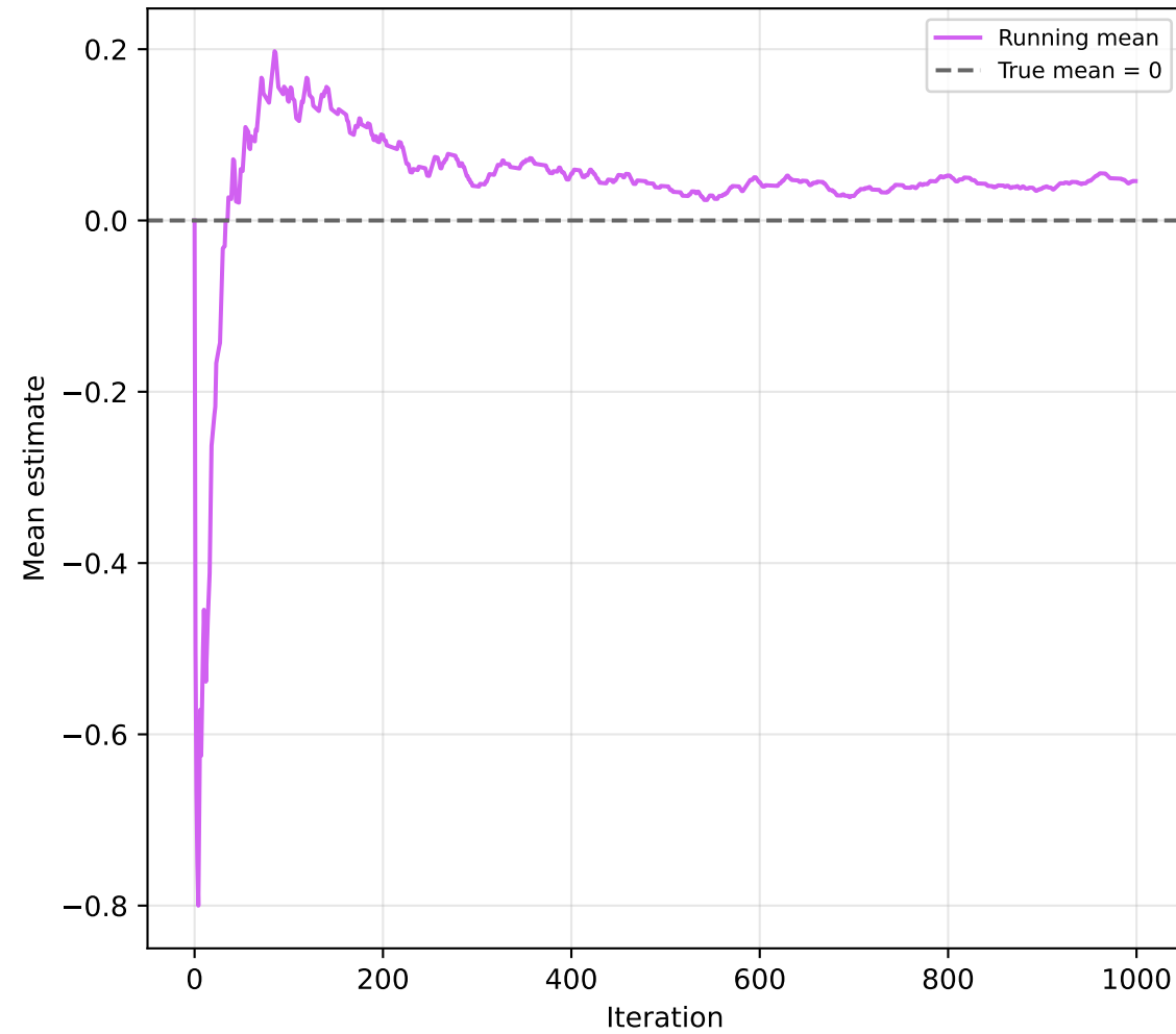
Running Mean: Random Walk
