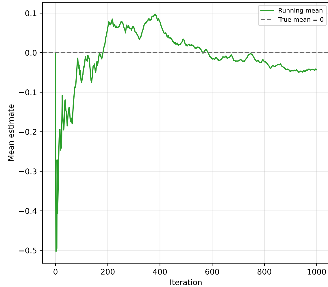
Running Mean: Normal
