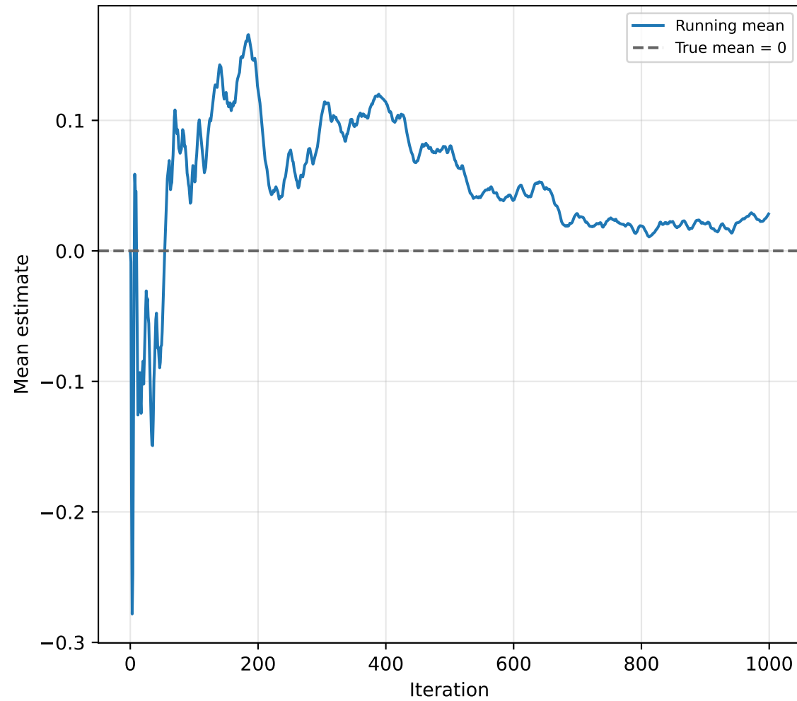
Running Mean: Uniform
